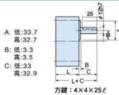
方鍵: 4×4×25ℓ
