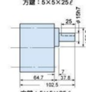
方鍵: 5×5×25ℓ
