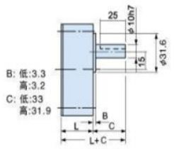
方鍵: 4×4×25ℓ
